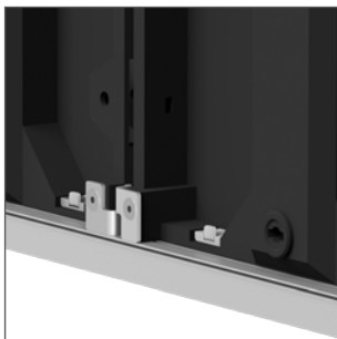
LED tiles are fixed with adaptors in the system groove.
